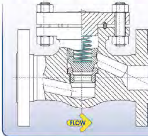
SPRING ASSISTED PISTON CHECK VALVE
