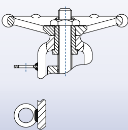
LOCKING FACILITY
