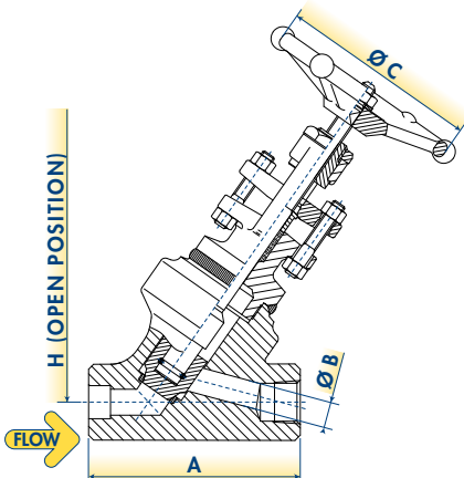
DESIGN TYPE W1 HANDWHEEL OPERATED AND V-GROOVE SEAL WELD BODY-BONNET CONNECTION
