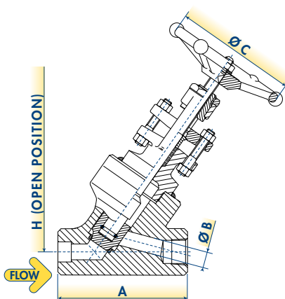
DESIGN TYPE W2 HANDWHEEL OPERATED AND TEE JOINT FILLED WELD BODY-BONNET CONNECTION
