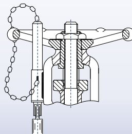
LOCKING DEVICE
