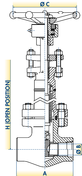
DESIGN TYPE P5 HANDWHEEL OPERATED WITH THRUST BEARINGS & RING JOINT GASKET BODY-BONNET CONNECTION
