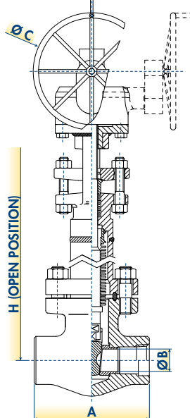
DESIGN TYPE P6 GEAR OPERATED & RING JOINT GASKET BODY-BONNET CONNECTION
