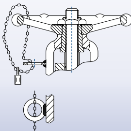
LOCKING FACILITY WITH C&P
