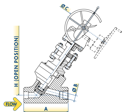
DESIGN TYPE W4 GEAR OPERATED AND TEE JOINT FILLED WELD BODY-BONNET CONNECTION
