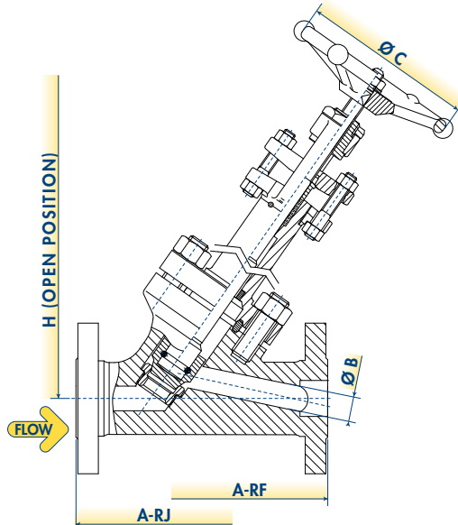
DESIGN TYPE S2 RING JOINT BODY-BONNET CONNECTION
