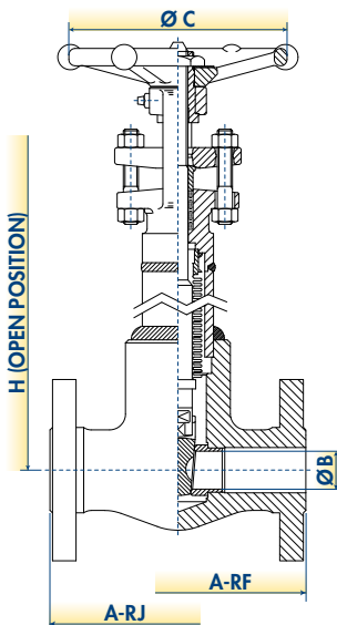
DESIGN TYPE P1 HANDWHEEL OPERATED
