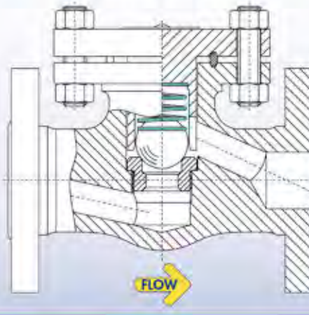
SPRING ASSISTED BALL CHECK VALVE
