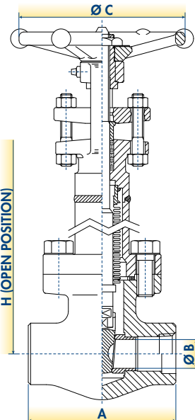
DESIGN TYPE P4 HANDWHEEL OPERATED & SPIRAL WOUND GASKET BODY-BONNET CONNECTION
